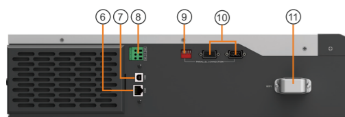
(3KW-5.5KW parallel model)
